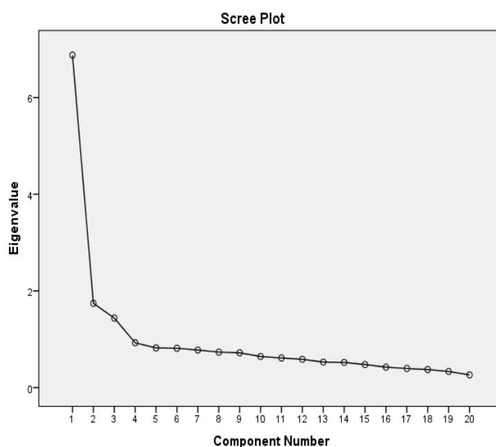
Figure 1: Eigenvalue graph of ATSS
