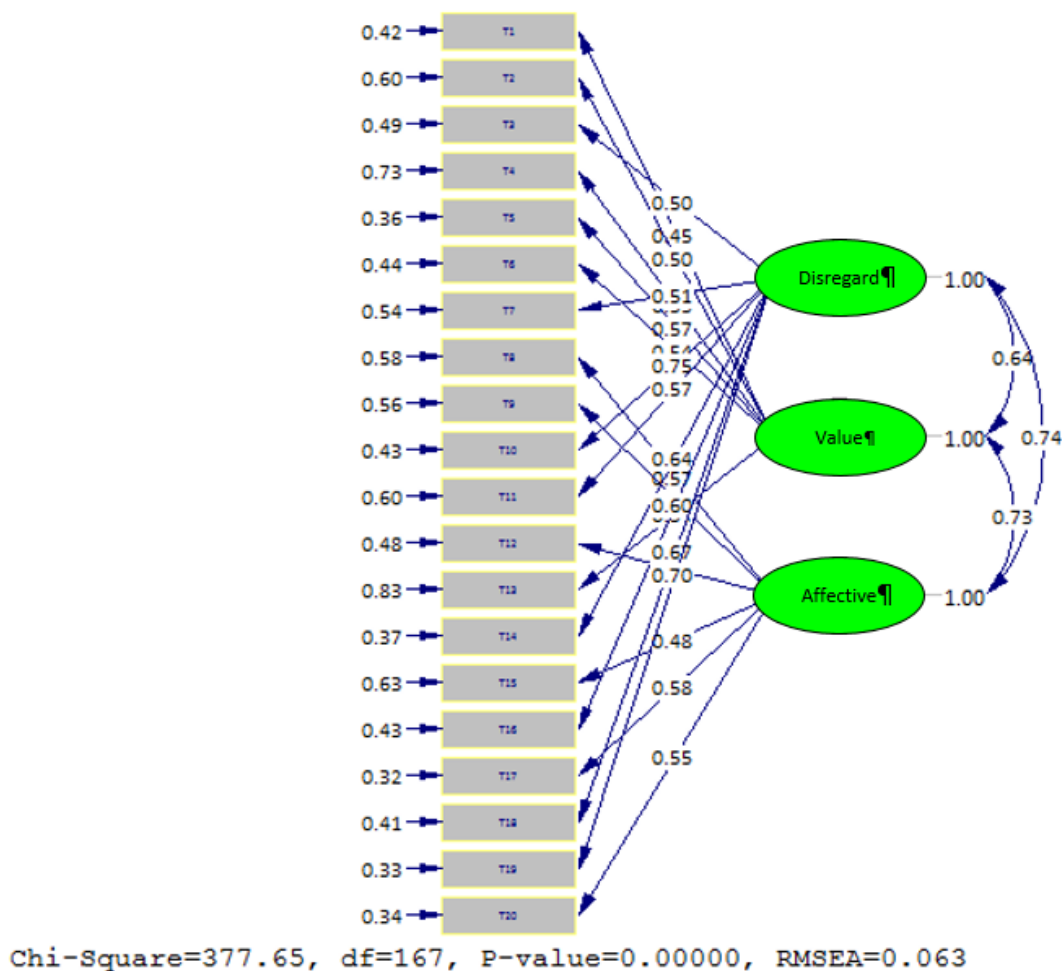
Figure 2: CFA for ATSS
